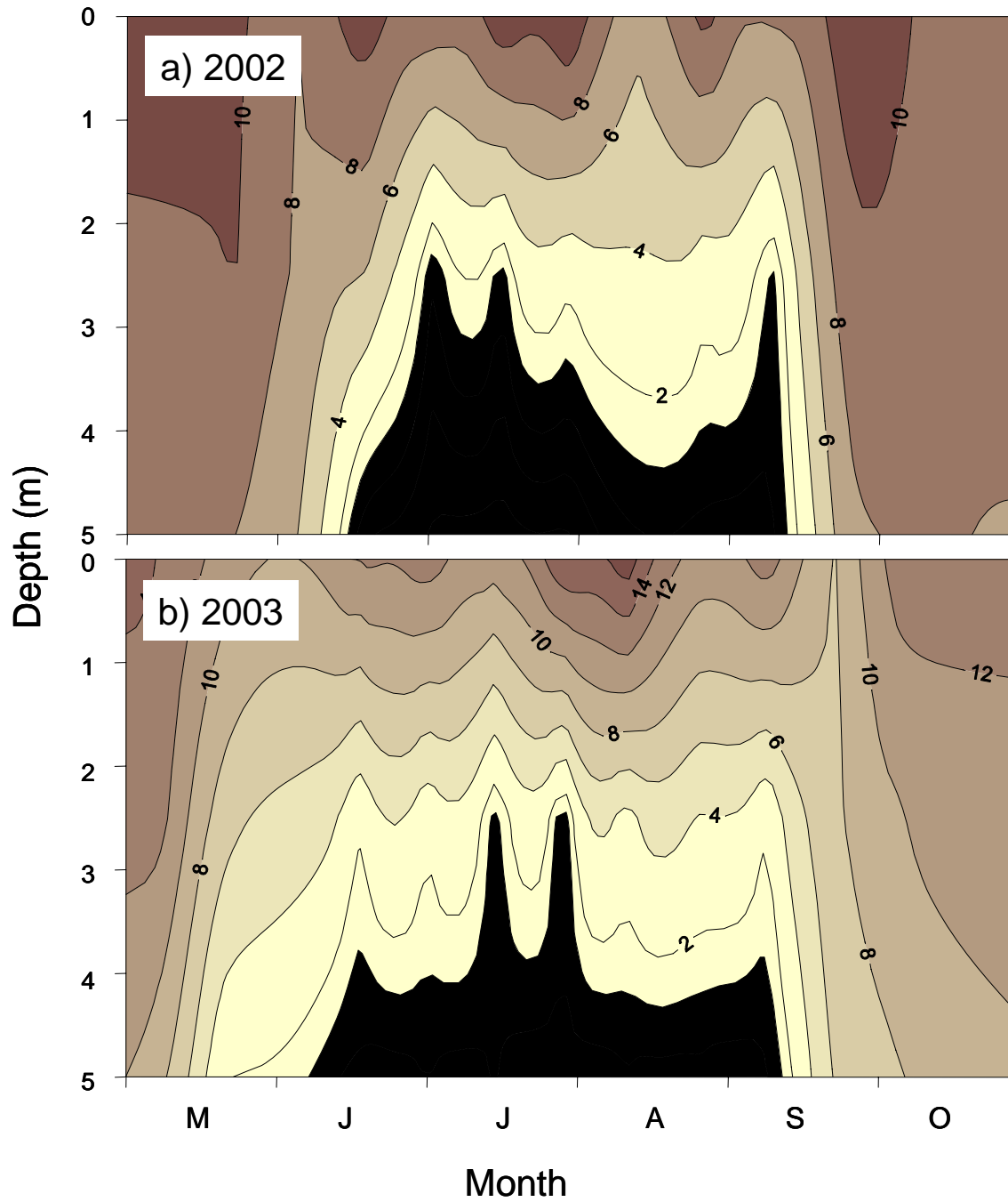
Figure 7. Seasonal and vertical dissolved oxygen (mg L -1 ) contours at station 10. Black shaded area represents concentrations < 1 mg L -1 .
