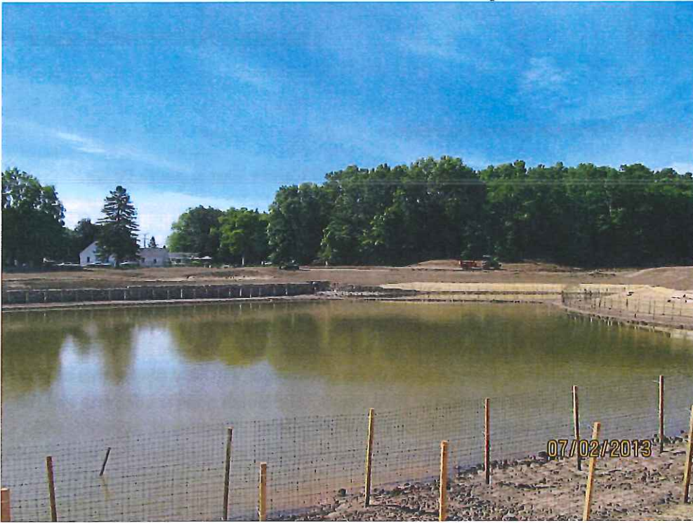
South Pond – Construction complete, exclusion fence & wetland plants in place, seeding completed.
