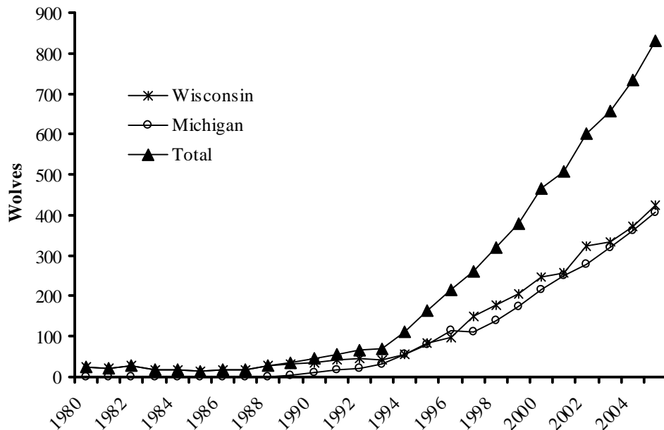
Figure 1-3. Wolf population estimates for Wisconsin, Michigan, and Wisconsin and Michigan combined (total) from 1980 - 2005.
