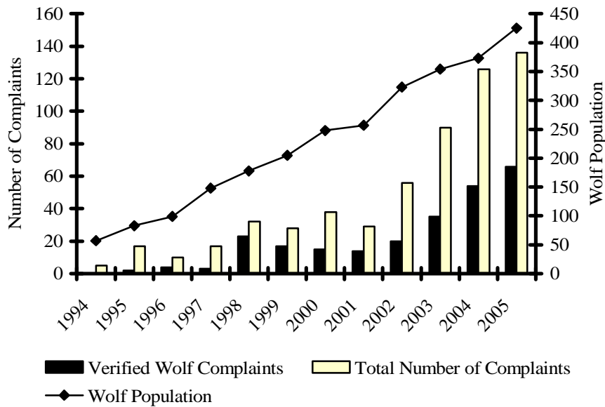
Figure 1-4. Annual wolf depredation complaints and annual minimum wolf population estimates in Wisconsin.
