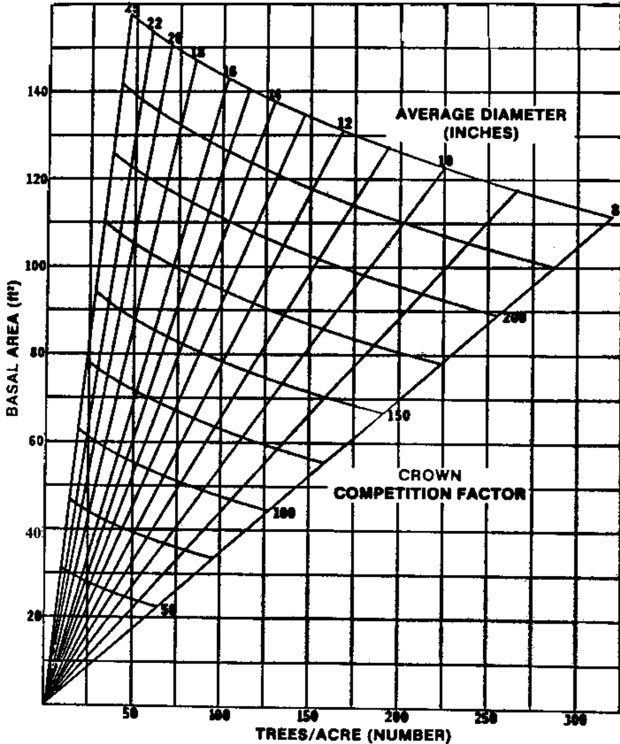
Figure 45.4. Black walnut stocking per acre for tree 8 to 25 inches in diameter (Schlesinger and Funk, 1977).
