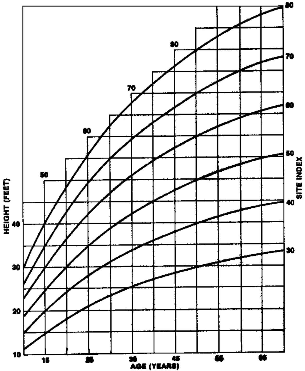
Figure 45.2. Site index curves for black walnut (Schlesinger and Funk 1977).
