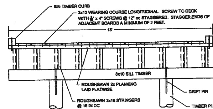
TYP SECTION THROUGH BOARDWALK AT PIER
