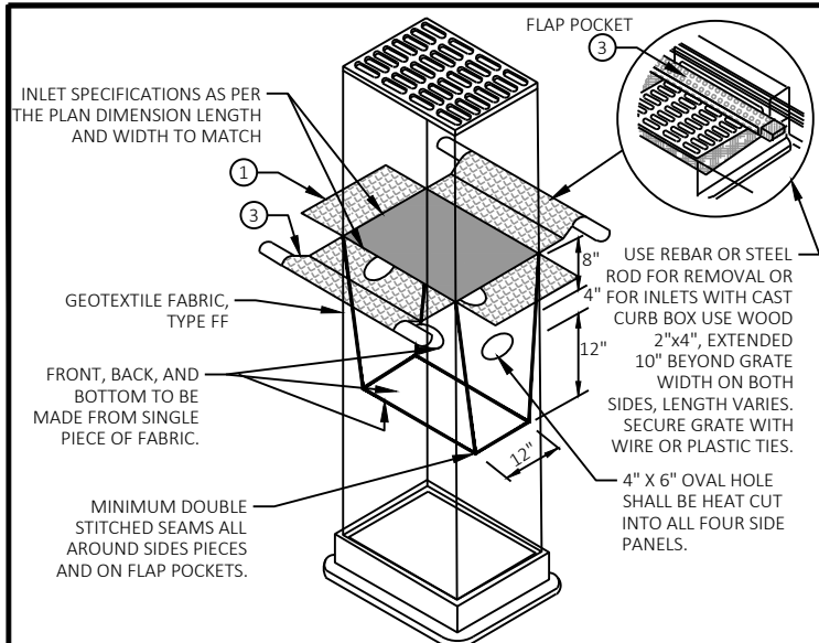
A INLET PROTECTION TYPE D 2.00 NOT TO SCALE
