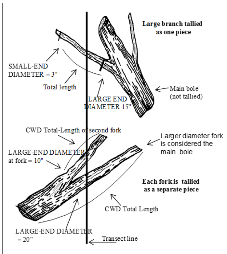
Figure 17. CWD tally rules for forked trees.
