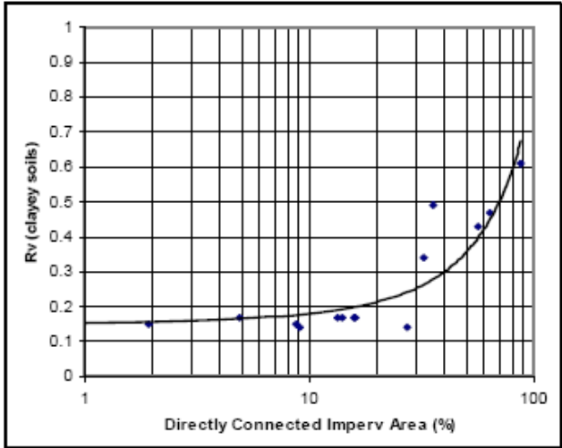
Figure xx.6 Relationships between the directly connected impervious area (%) and the calculated volumetric runoff coefficients (Rv) for each land use category for clayey soil (Bochis and Pitt 2005)
