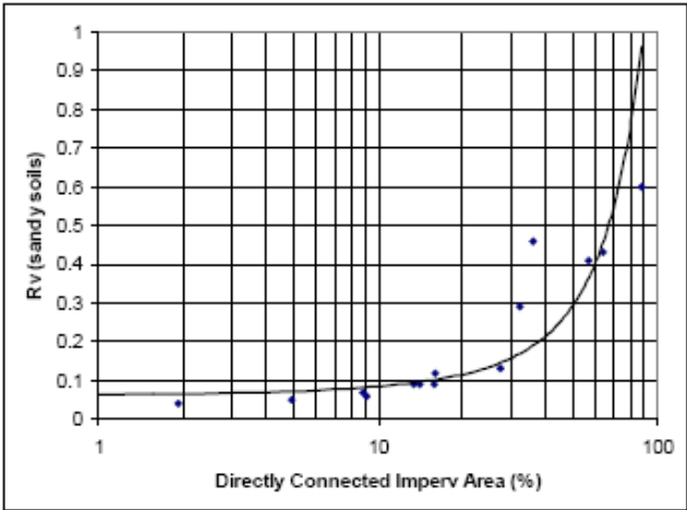
Figure xx.5 Relationships between the directly connected impervious area (%) and the calculated volumetric runoff coefficients (Rv) for each land use category for sandy soil (Bochis and Pitt 2005)
