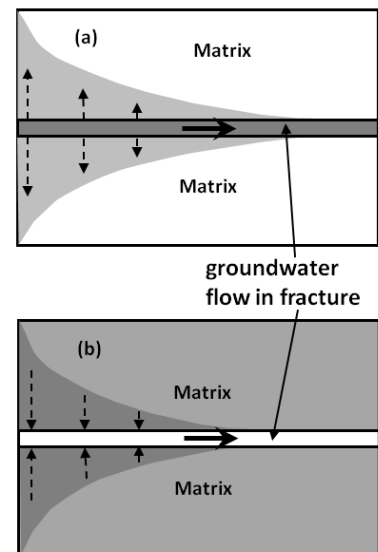
(a) When concentrations are higher in the fracture, solutes diffuse from the fracture into the matrix. (b) When concentrations are higher in the matrix, solutes diffuse from the matrix into the fracture.
